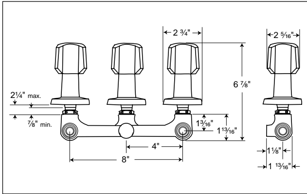
Three Valve Tub/Shower with Acrylic Handles
