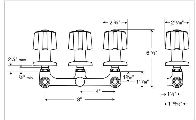
Three Valve Tub/Shower with Blade Handles
