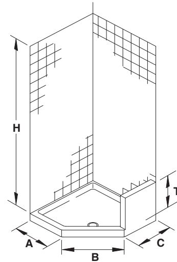
Note: All dimensions taken at centerline of ledge/threshold.
